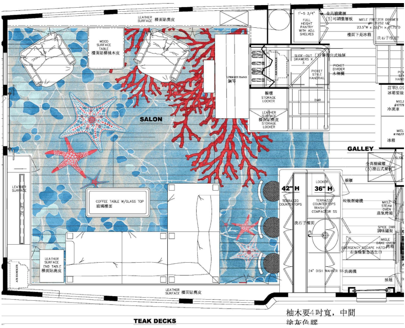
SHOPDRAWING
